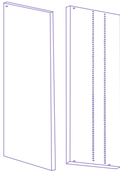
Island R/L Island Thru 12"W x 34-1/2"H x 24"D
